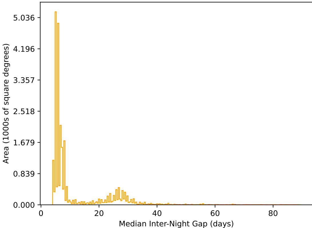
too_ignore_10_4v3.4_10yrs All sky r band: Median Inter-Night Gap
