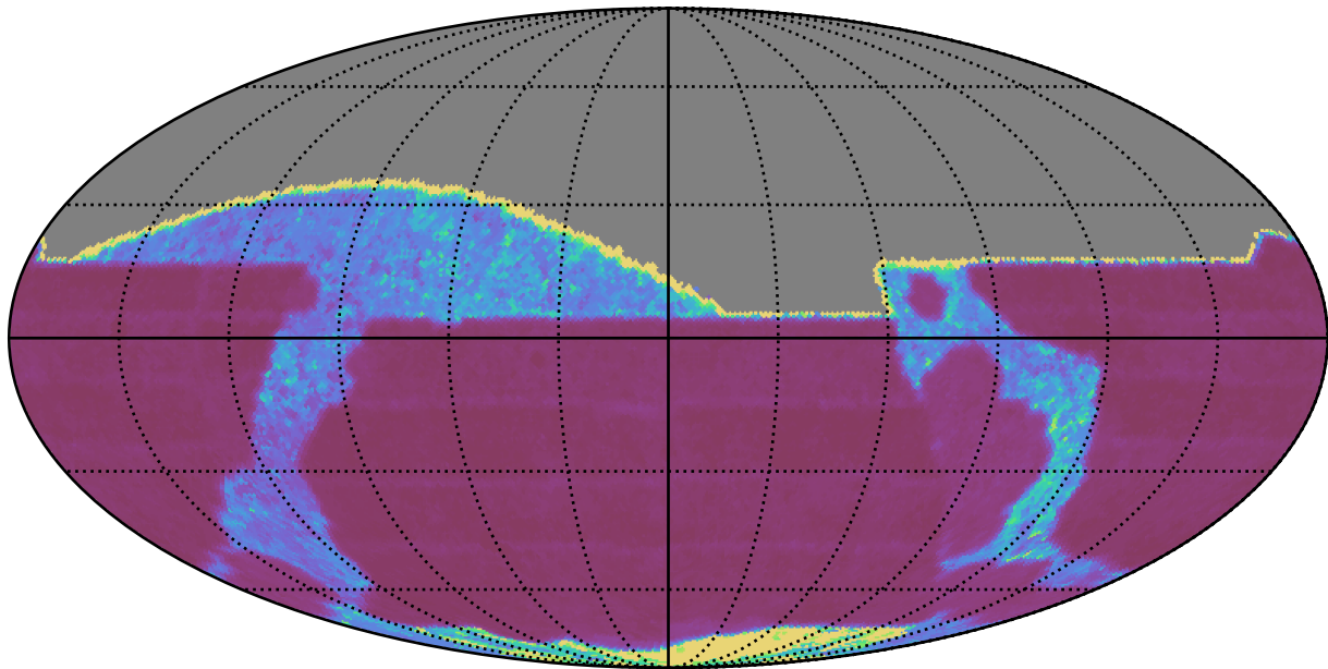
too_ignore_10_4v3.4_10yrs All sky i band: Median Inter-Night Gap
