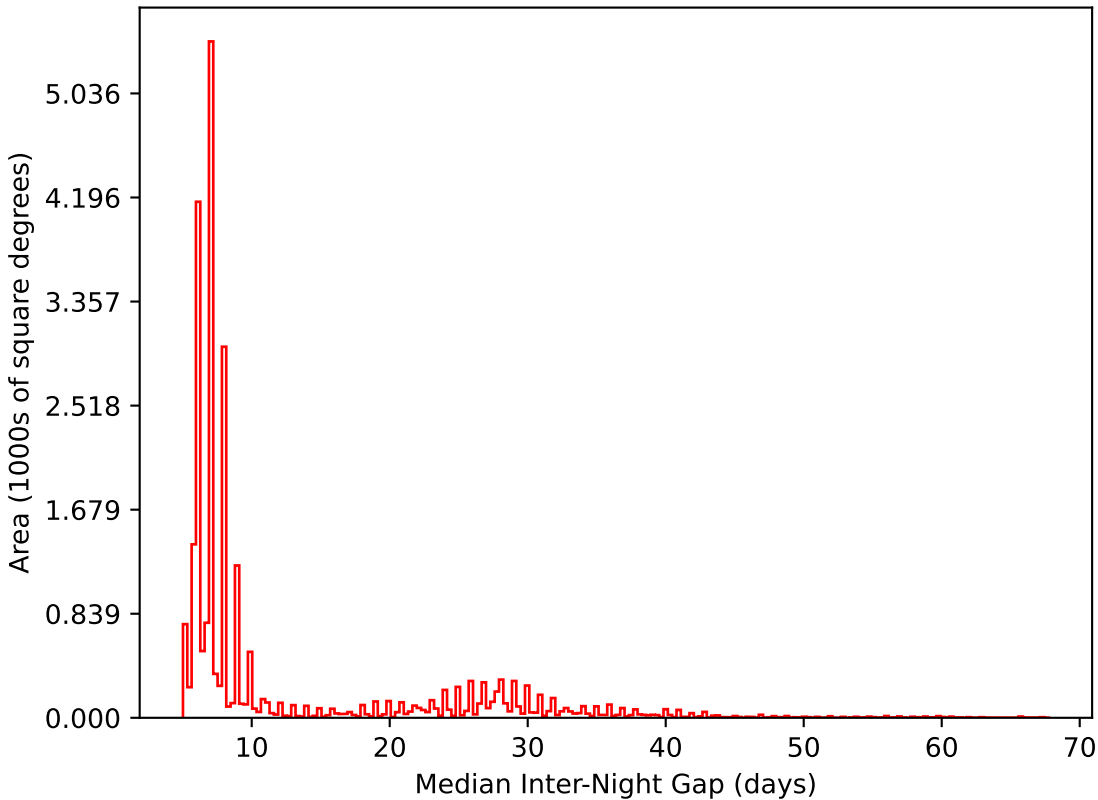
too_ignore_10_4v3.4_10yrs All sky i band: Median Inter-Night Gap
