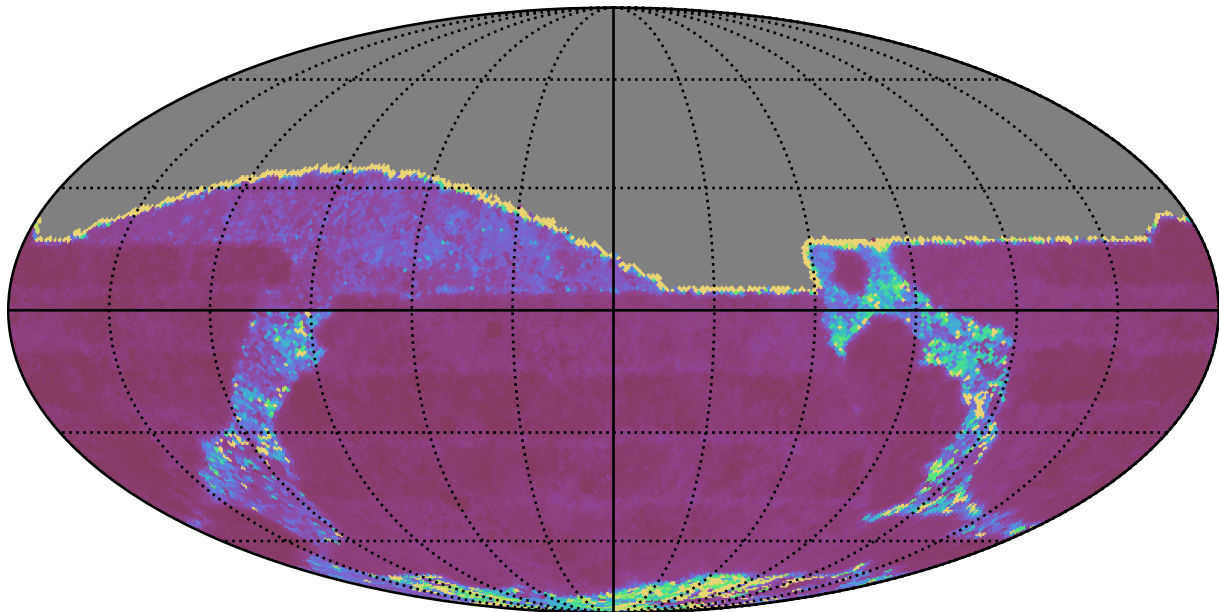
too_ignore_10_4v3.4_10yrs All sky g band: Median Inter-Night Gap
