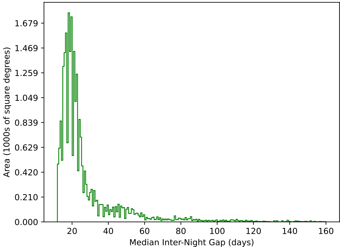
too_ignore_10_4v3.4_10yrs All sky g band: Median Inter-Night Gap
