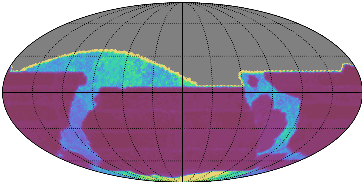
too_ignore_10_4v3.4_10yrs All sky all bands: Median Inter-Night Gap
