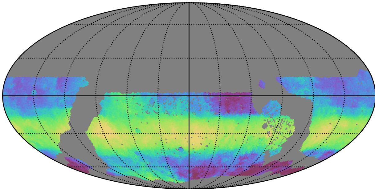
too_ignore_10_4v3.4_10yrs WFD z band: Median HA
