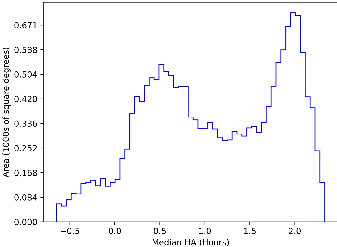
too_ignore_10_4v3.4_10yrs WFD z band: Median HA
