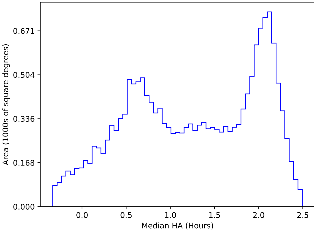
too_ignore_10_4v3.4_10yrs WFD y band: Median HA
