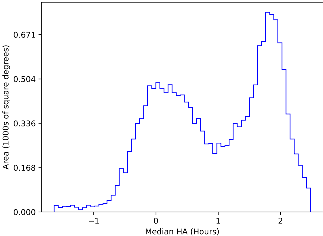
too_ignore_10_4v3.4_10yrs WFD u band: Median HA
