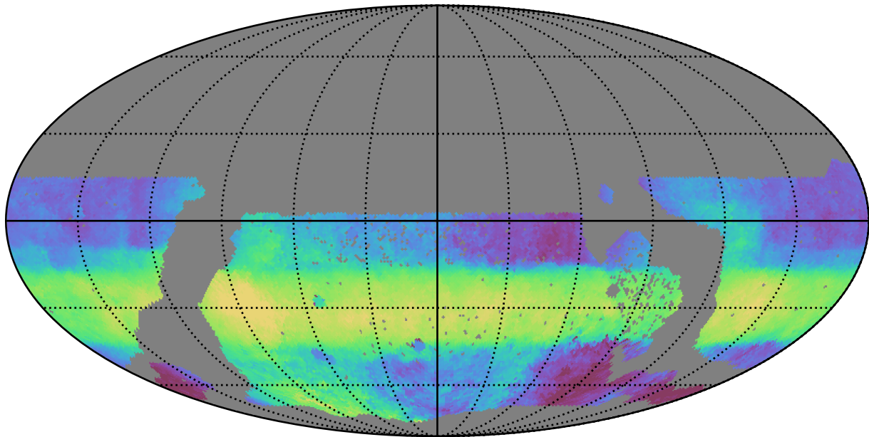
too_ignore_10_4v3.4_10yrs WFD r band: Median HA
