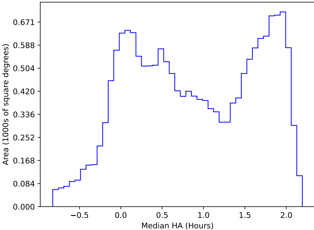
too_ignore_10_4v3.4_10yrs WFD r band: Median HA
