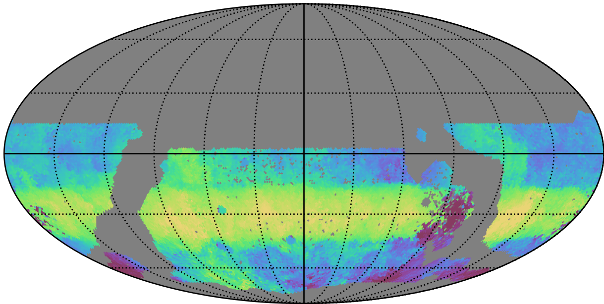
too_ignore_10_4v3.4_10yrs WFD g band: Median HA
