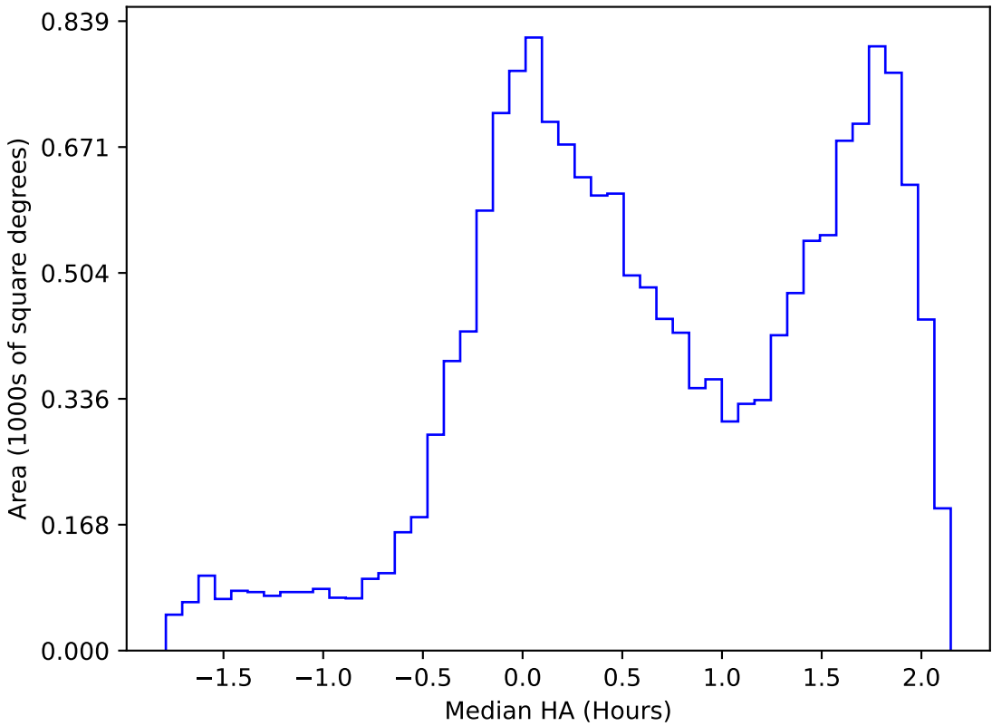
too_ignore_10_4v3.4_10yrs WFD g band: Median HA
