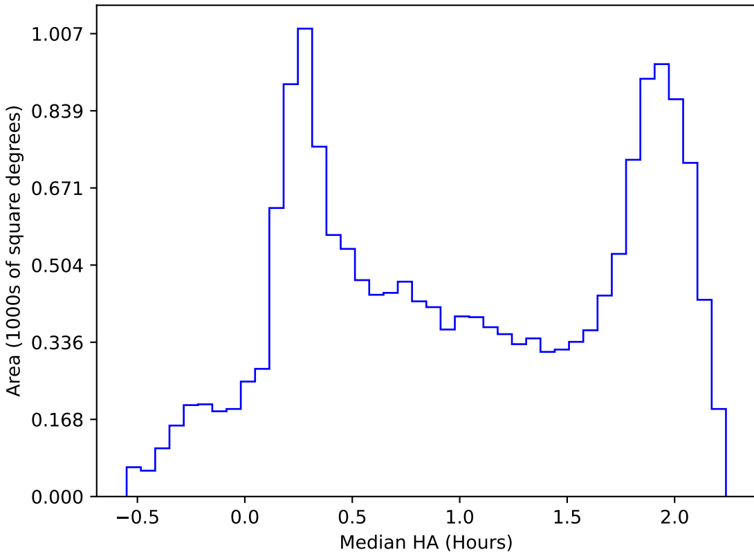
too_ignore_10_4v3.4_10yrs WFD all bands: Median HA
