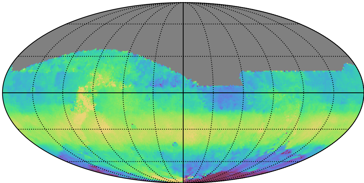
too_ignore_10_4v3.4_10yrs All sky z band: Median HA
