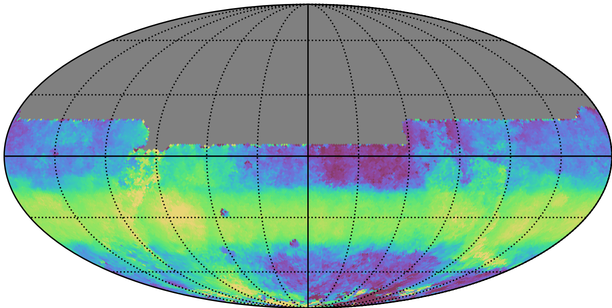
too_ignore_10_4v3.4_10yrs All sky y band: Median HA
