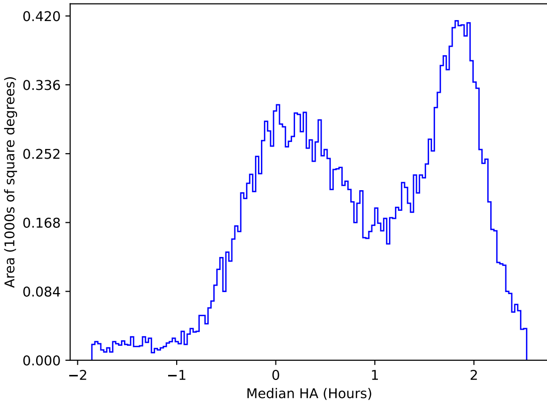
too_ignore_10_4v3.4_10yrs All sky u band: Median HA
