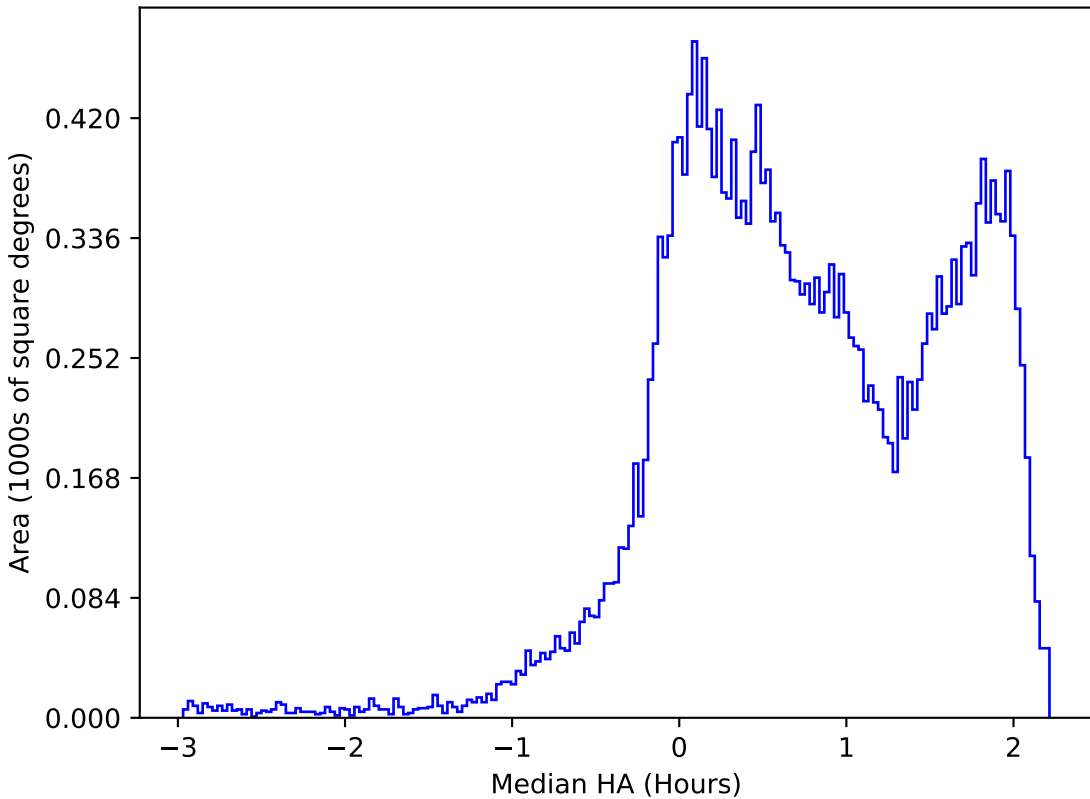
too_ignore_10_4v3.4_10yrs All sky r band: Median HA
