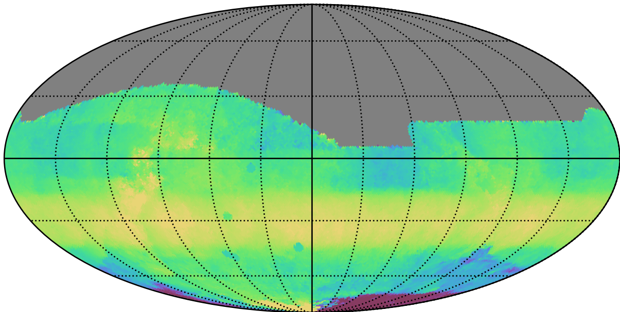
too_ignore_10_4v3.4_10yrs All sky i band: Median HA
