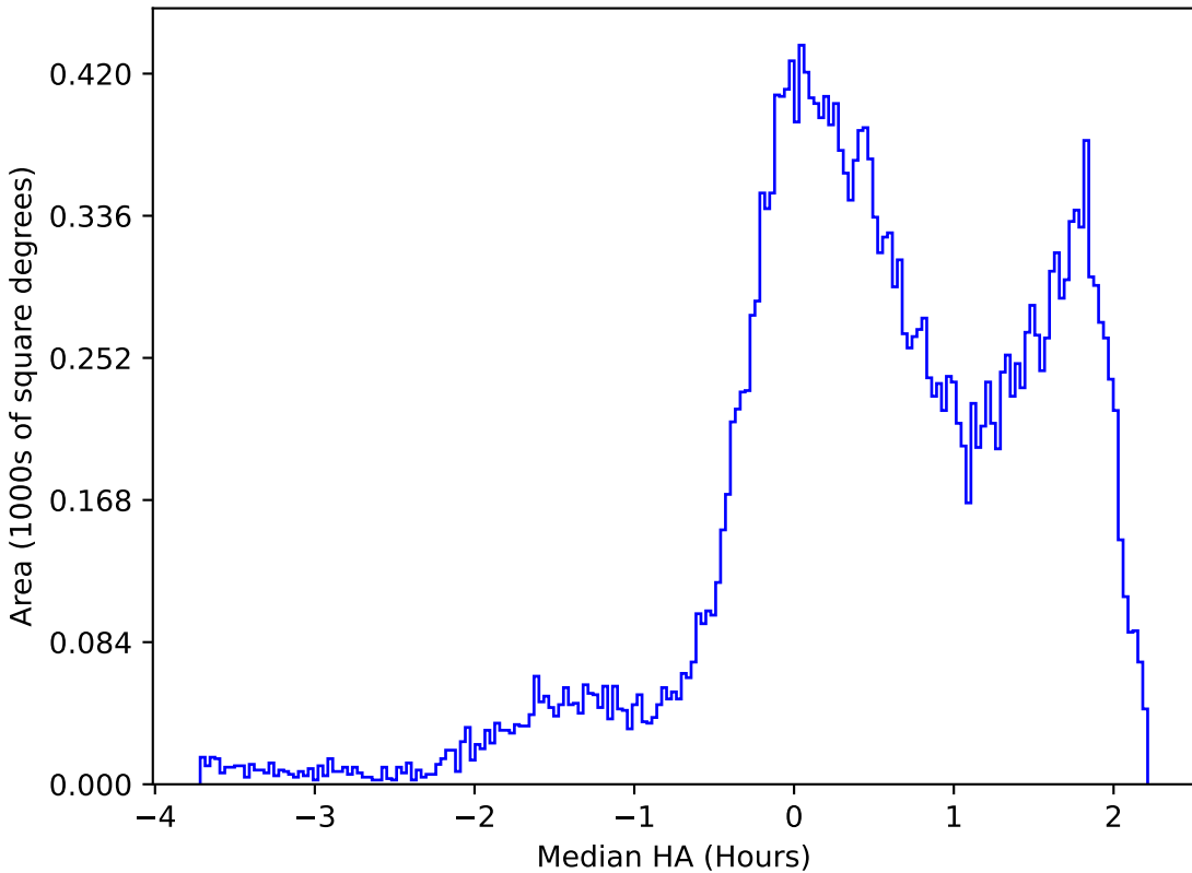
too_ignore_10_4v3.4_10yrs All sky g band: Median HA
