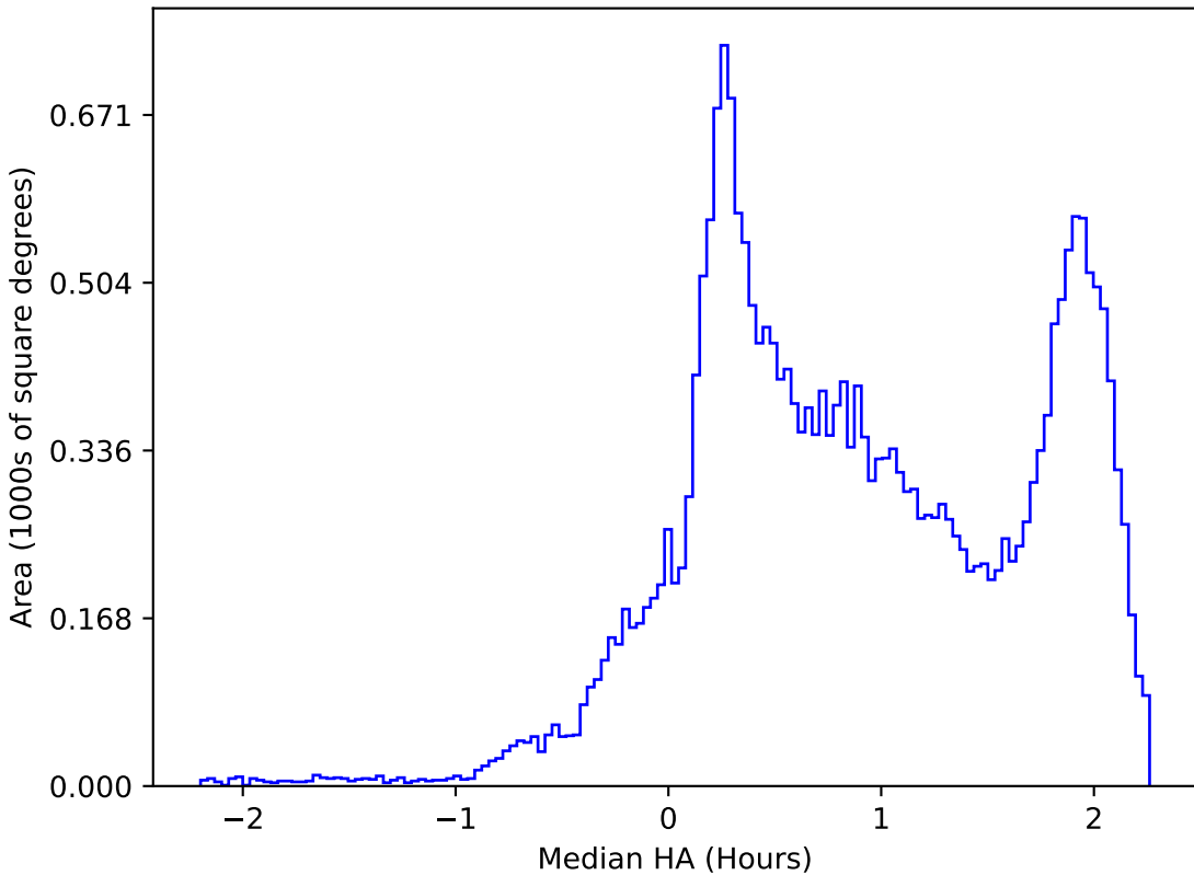
too_ignore_10_4v3.4_10yrs All sky all bands: Median HA
