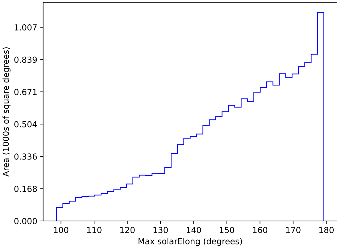
too_ignore_10_4v3.4_10yrs WFD z band: Max solarElong
