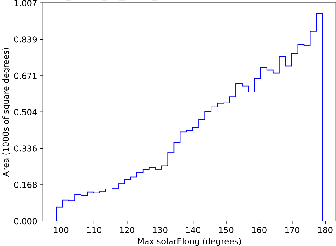
too_ignore_10_4v3.4_10yrs WFD y band: Max solarElong
