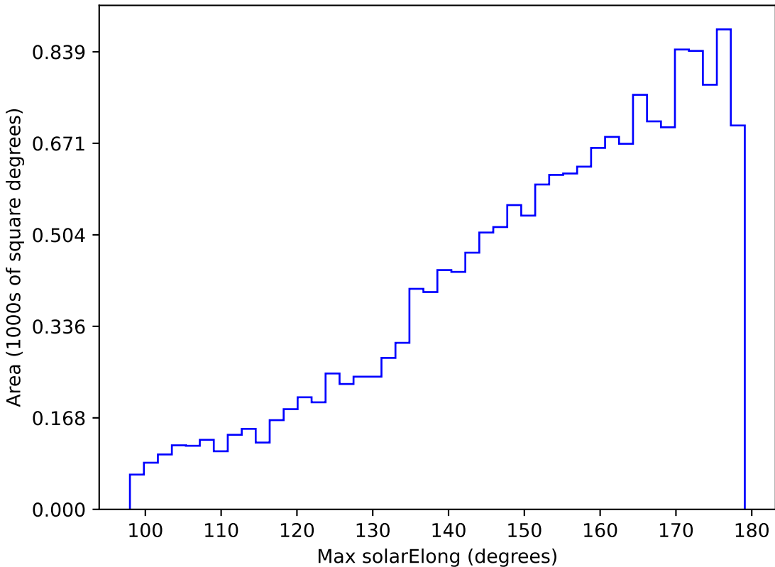
too_ignore_10_4v3.4_10yrs WFD u band: Max solarElong
