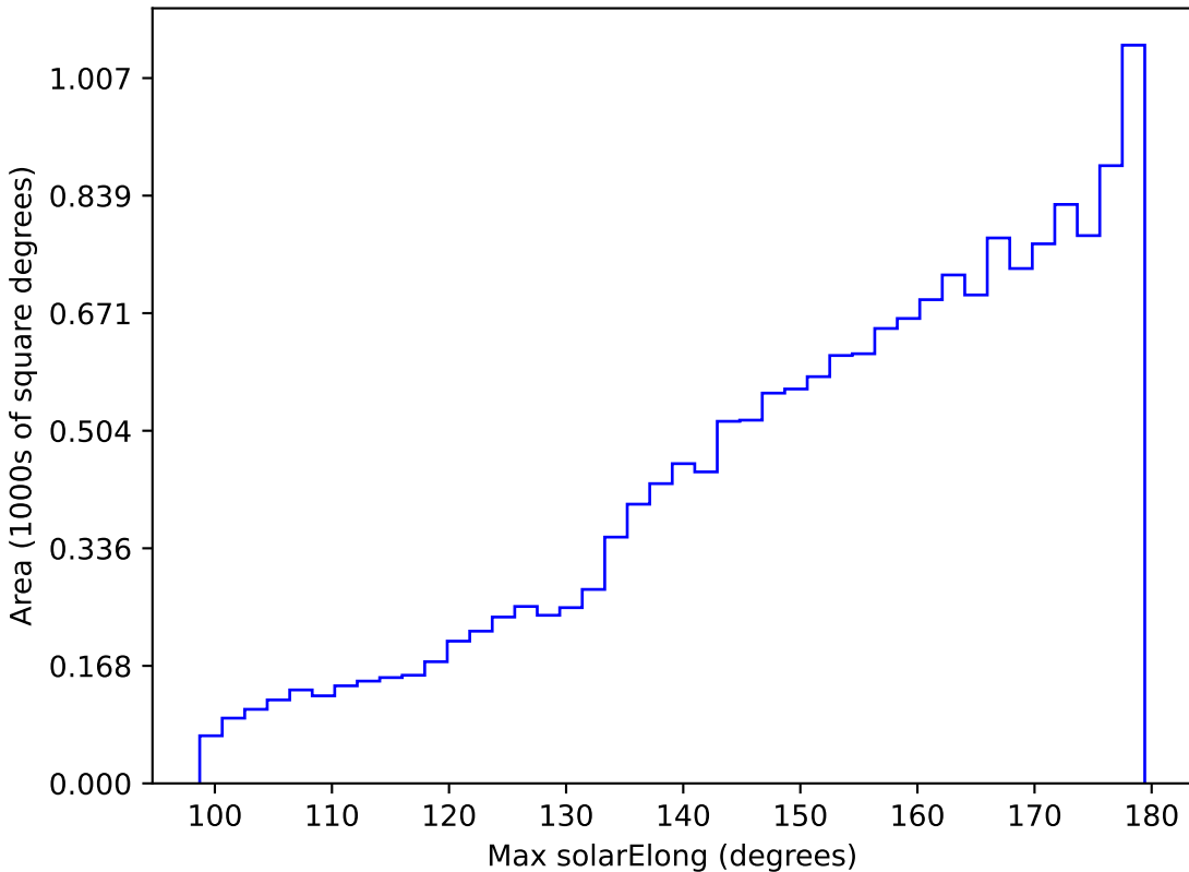
too_ignore_10_4v3.4_10yrs WFD i band: Max solarElong
