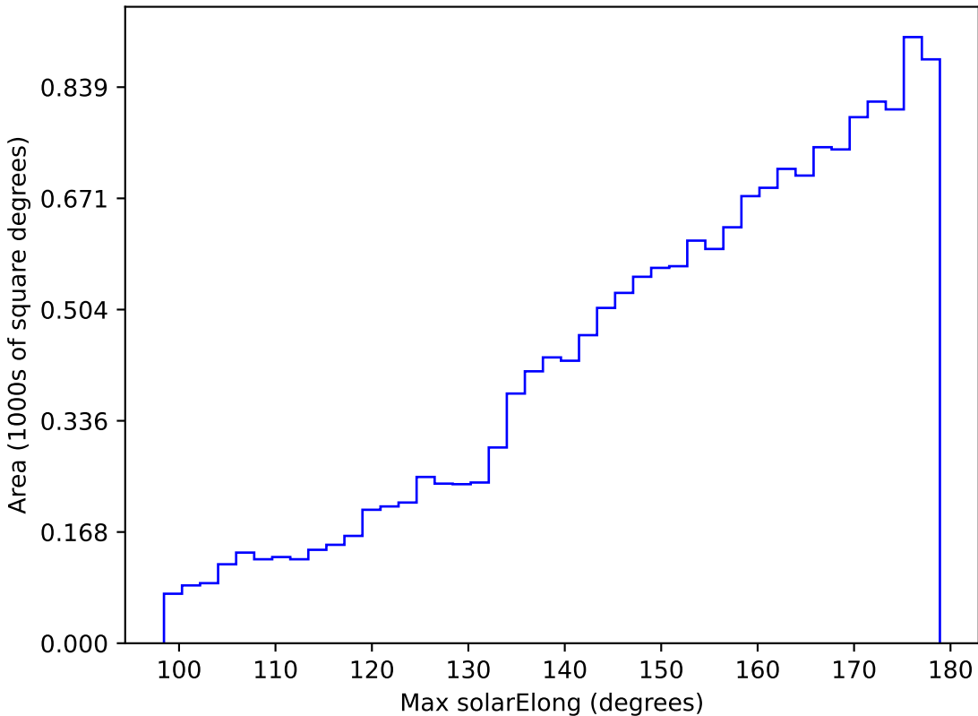
too_ignore_10_4v3.4_10yrs WFD g band: Max solarElong
