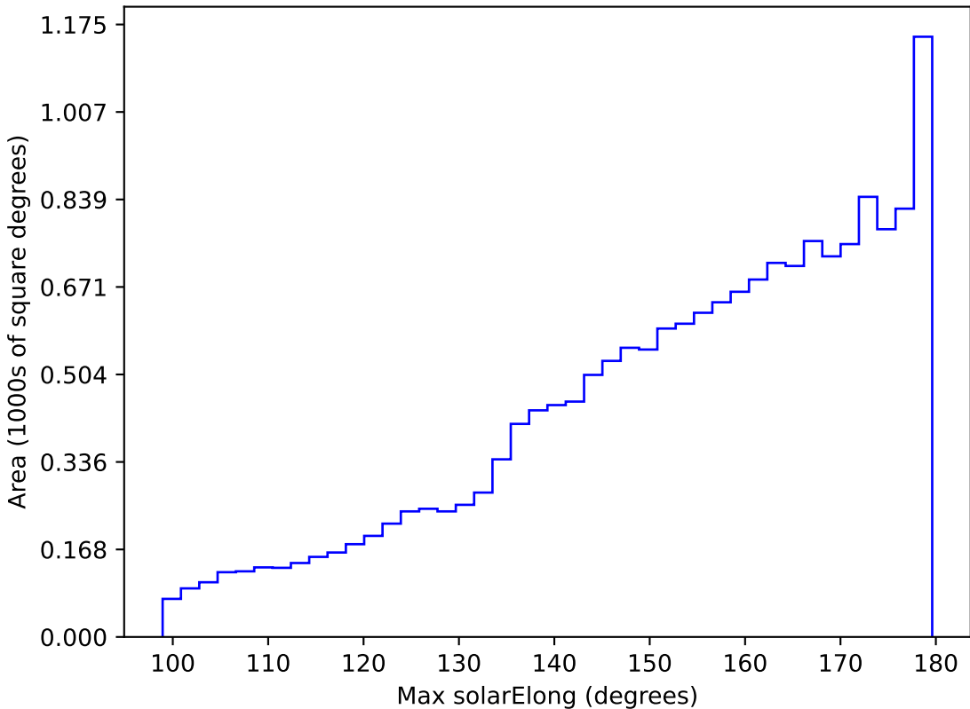
too_ignore_10_4v3.4_10yrs WFD all bands: Max solarElong
