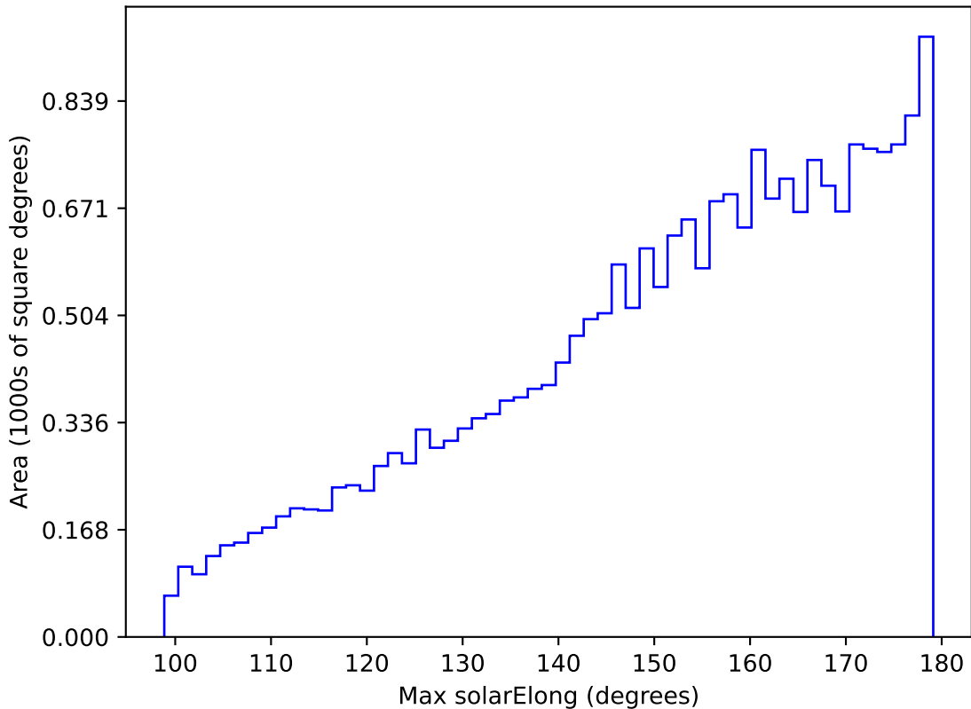
too_ignore_10_4v3.4_10yrs All sky y band: Max solarElong
