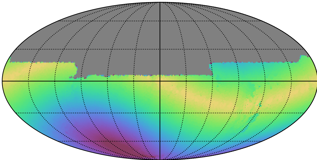
too_ignore_10_4v3.4_10yrs All sky u band: Max solarElong
