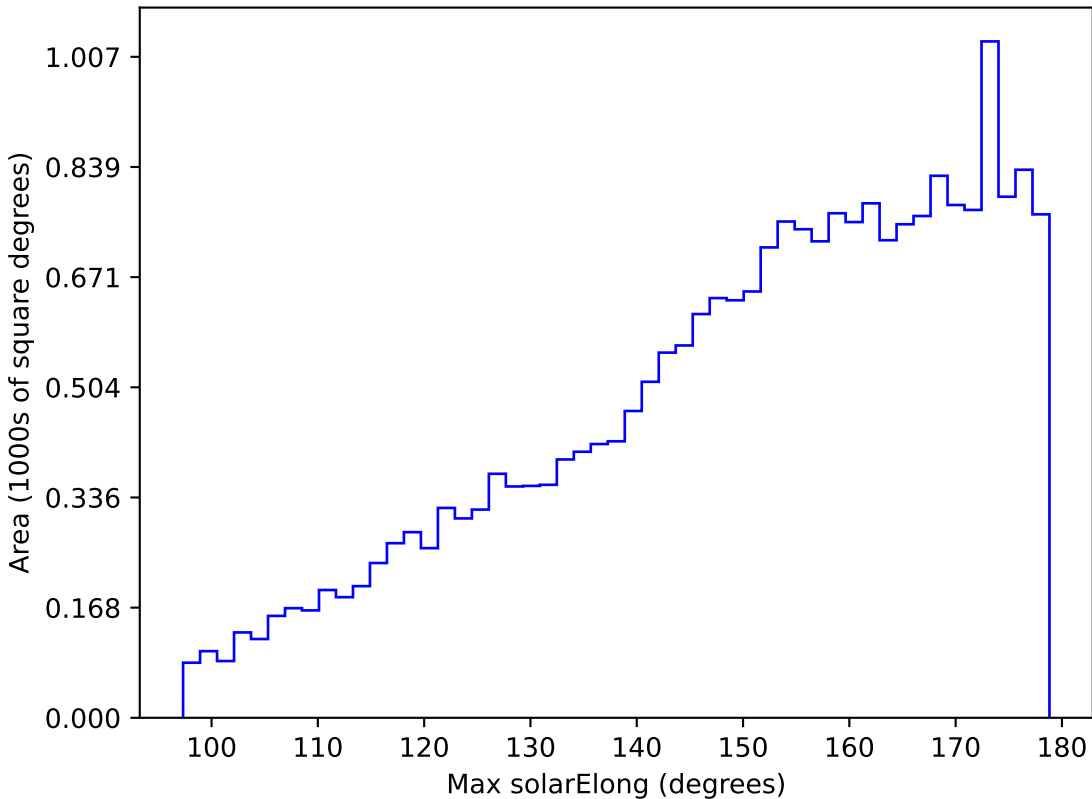
too_ignore_10_4v3.4_10yrs All sky u band: Max solarElong
