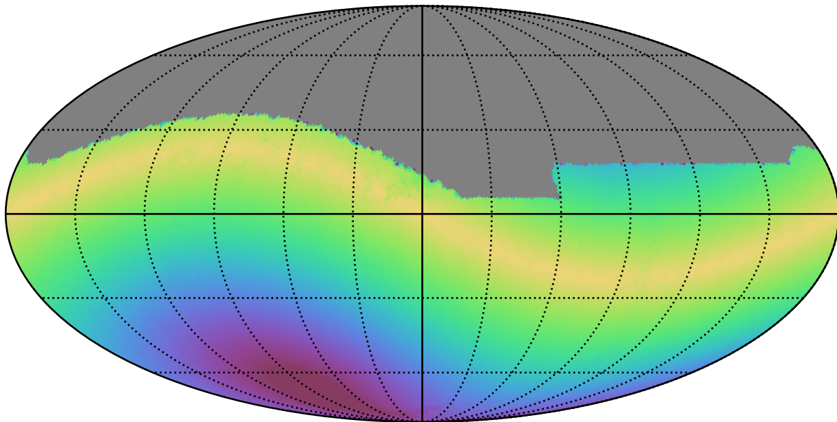
too_ignore_10_4v3.4_10yrs All sky r band: Max solarElong
