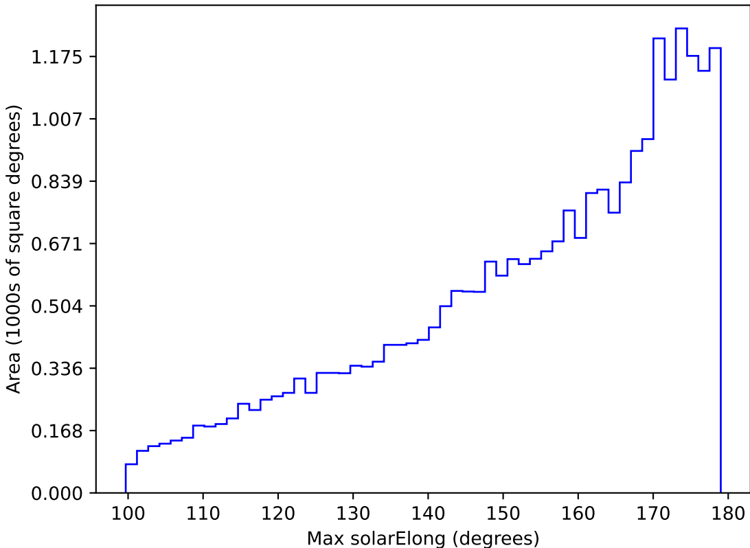
too_ignore_10_4v3.4_10yrs All sky g band: Max solarElong
