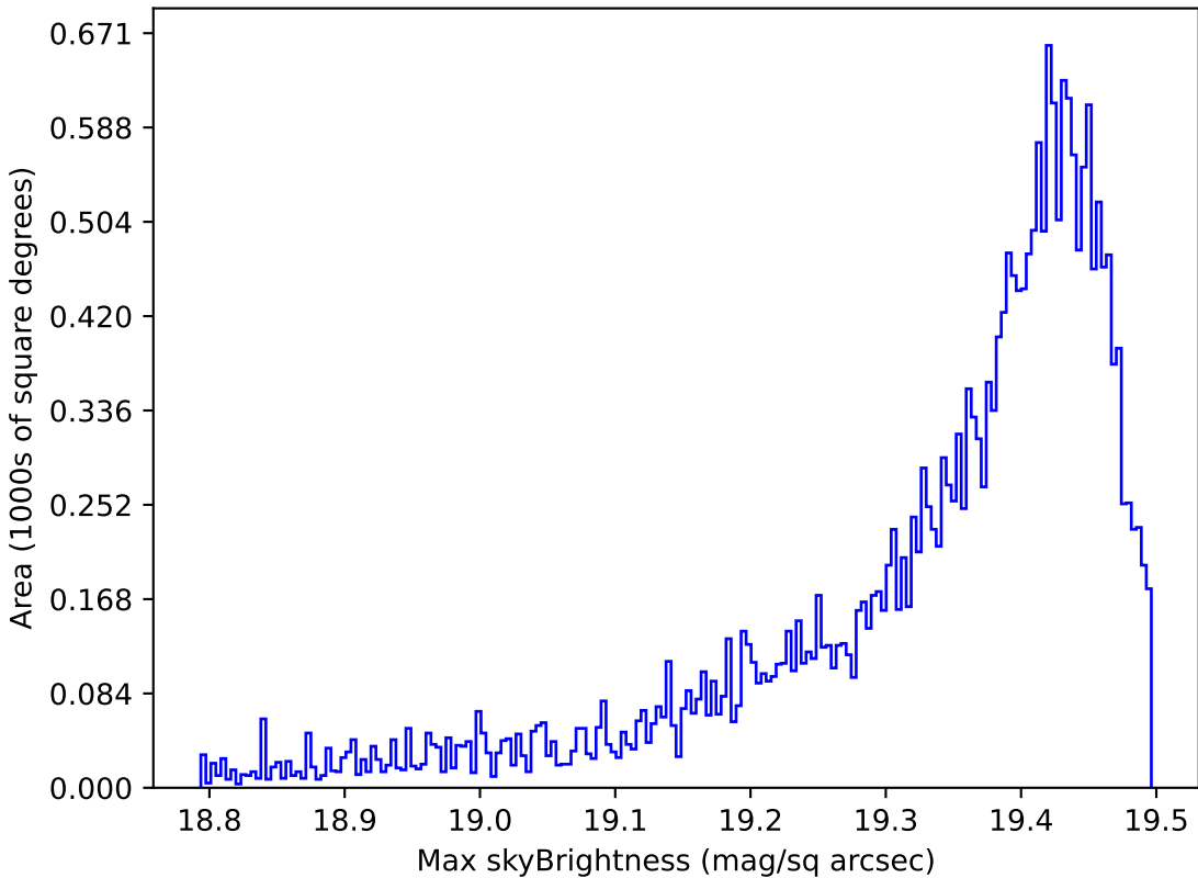
too_ignore_10_4v3.4_10yrs Yr 1 z band: Max skyBrightness
