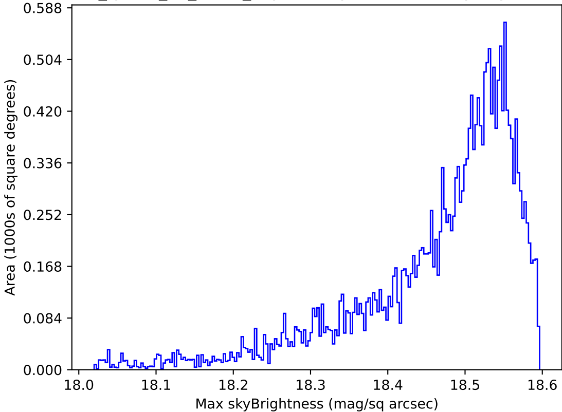
too_ignore_10_4v3.4_10yrs Yr 1 y band: Max skyBrightness
