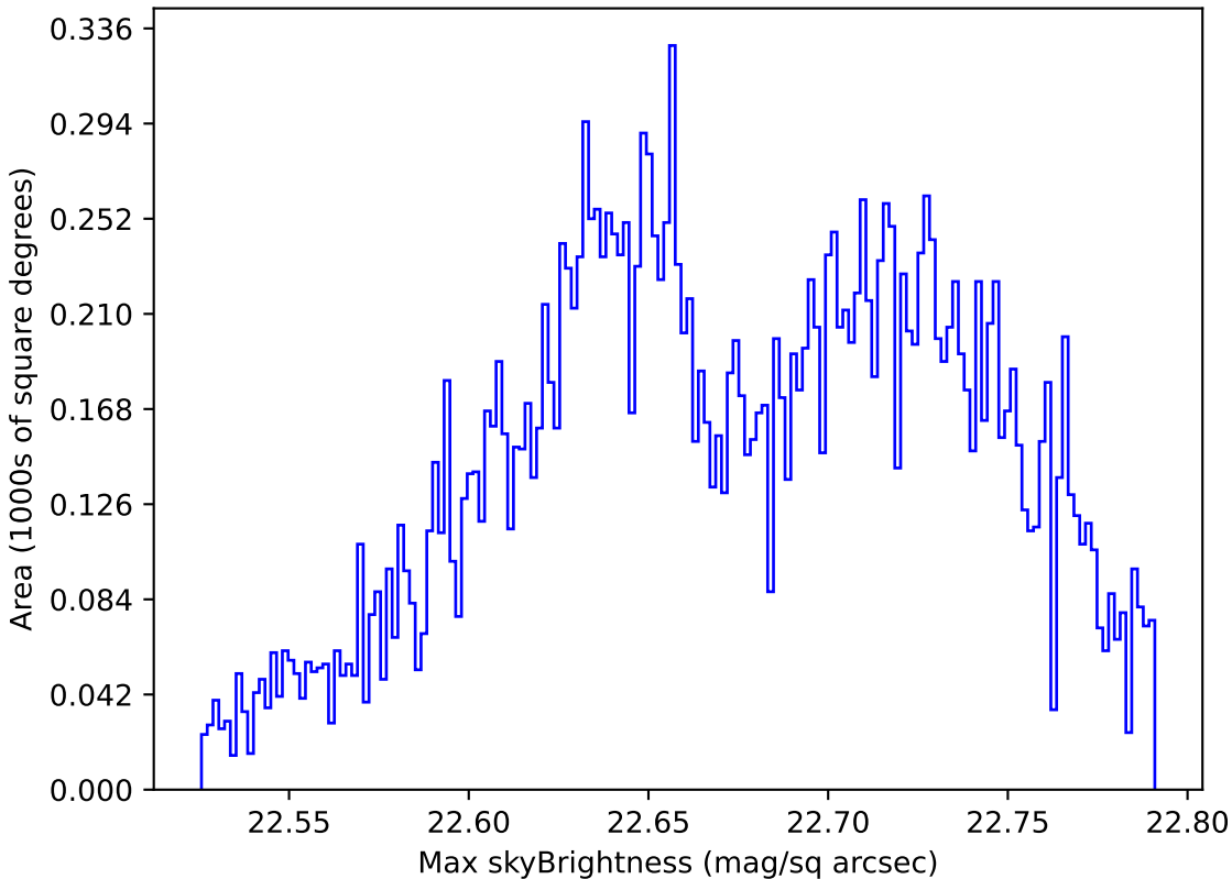
too_ignore_10_4v3.4_10yrs Yr 1 u band: Max skyBrightness
