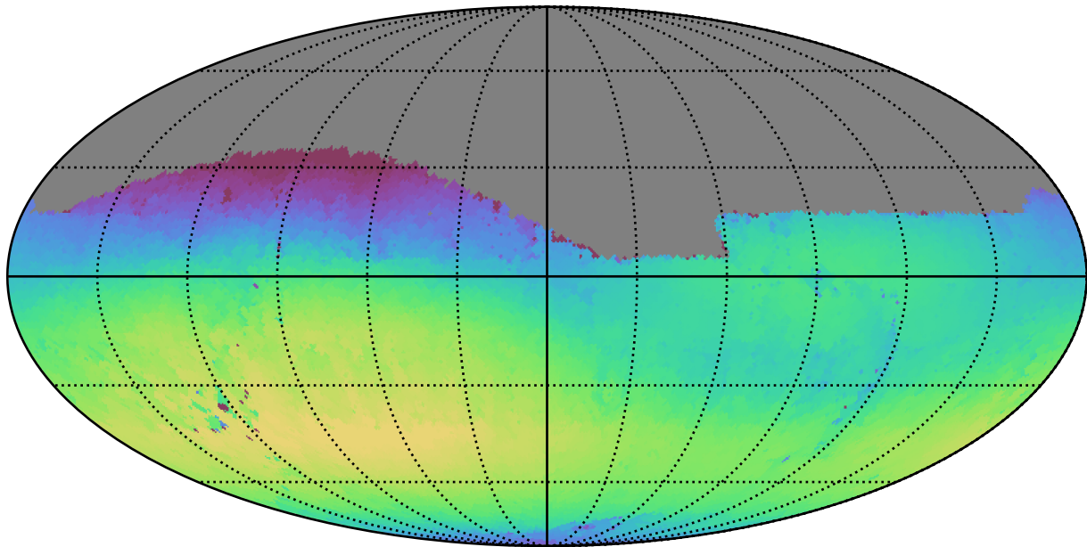
too_ignore_10_4v3.4_10yrs Yr 1 r band: Max skyBrightness
