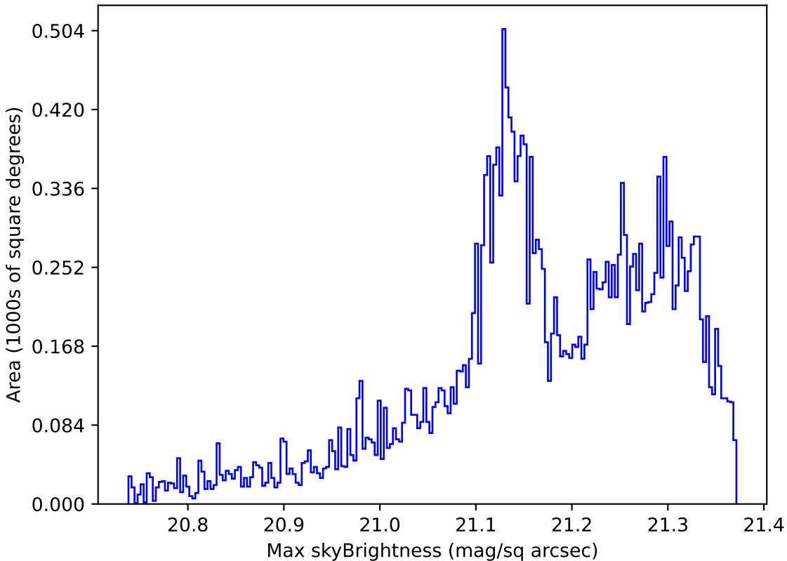
too_ignore_10_4v3.4_10yrs Yr 1 r band: Max skyBrightness
