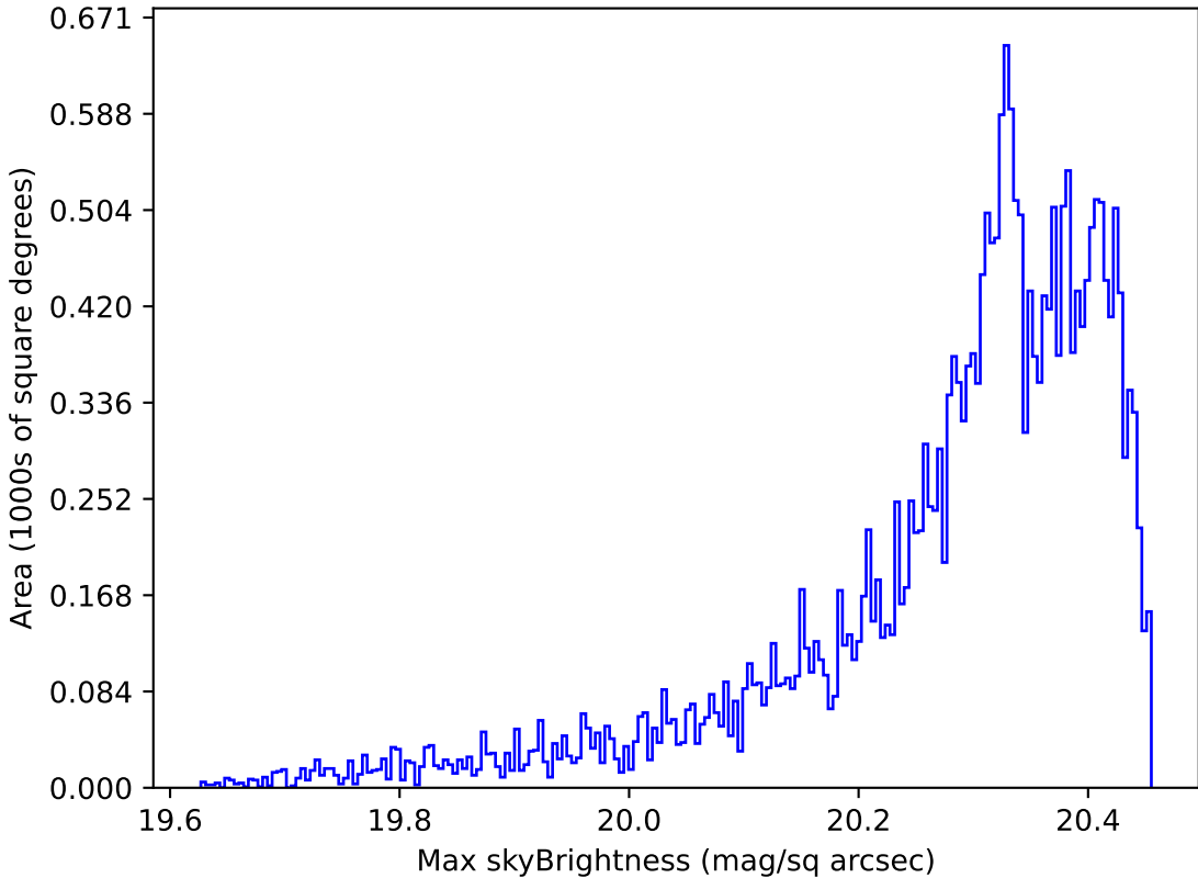
too_ignore_10_4v3.4_10yrs Yr 1 i band: Max skyBrightness
