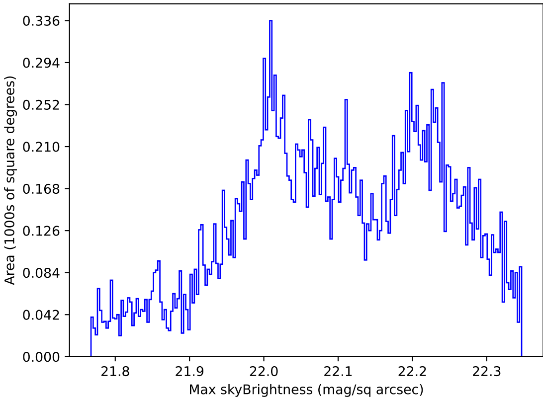
too_ignore_10_4v3.4_10yrs Yr 1 g band: Max skyBrightness
