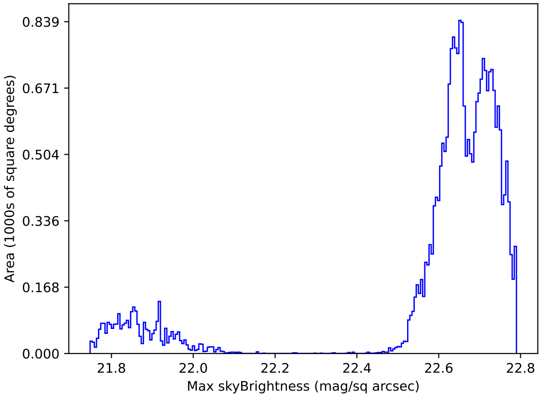
too_ignore_10_4v3.4_10yrs Yr 1 all bands: Max skyBrightness
