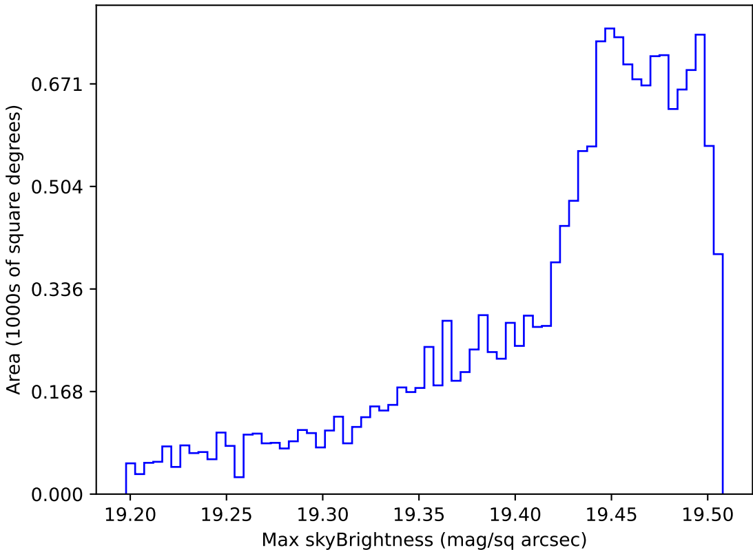
too_ignore_10_4v3.4_10yrs WFD z band: Max skyBrightness
