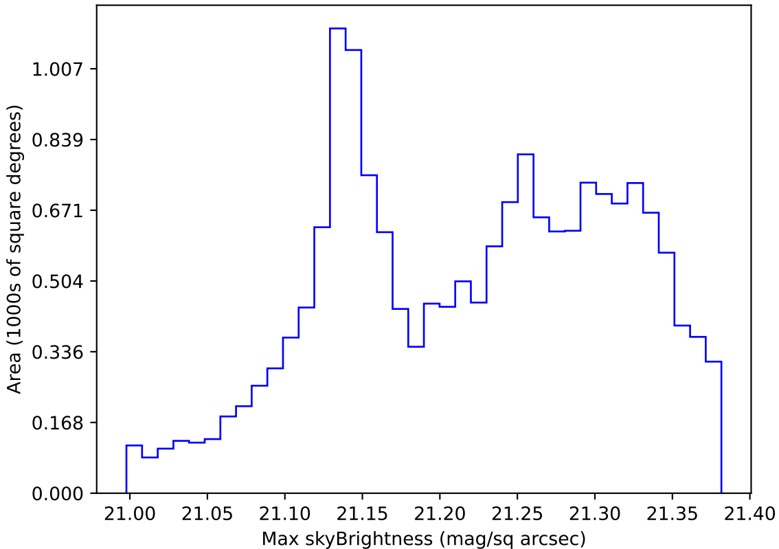
too_ignore_10_4v3.4_10yrs WFD r band: Max skyBrightness
