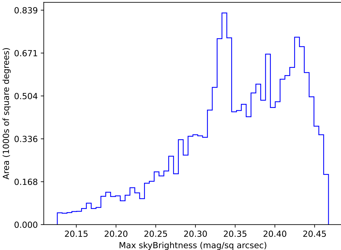
too_ignore_10_4v3.4_10yrs WFD i band: Max skyBrightness
