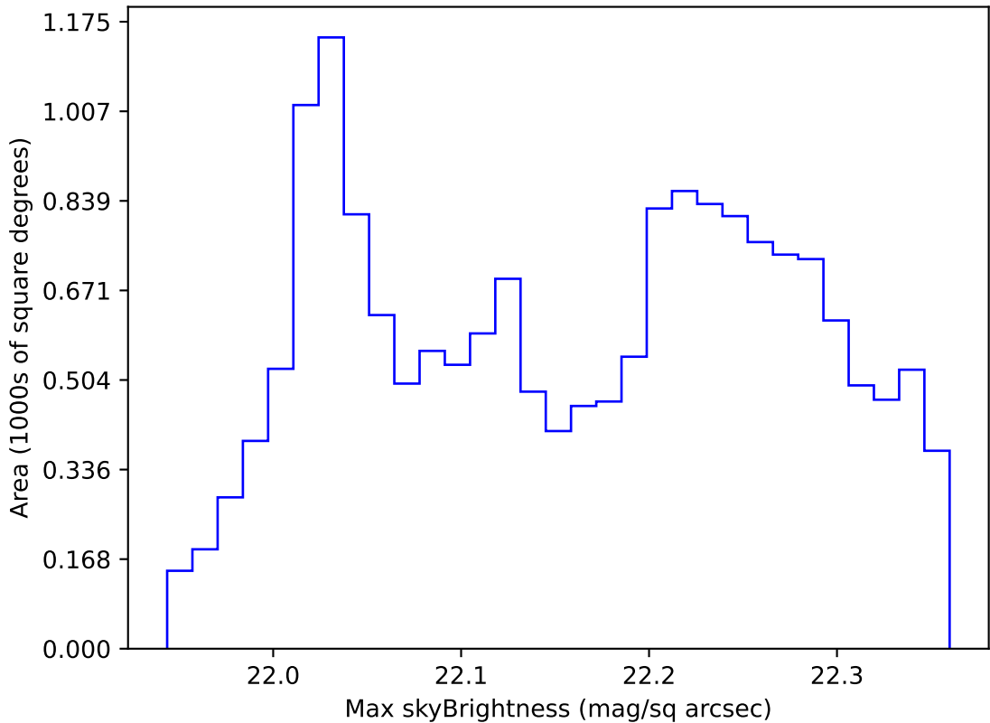
too_ignore_10_4v3.4_10yrs WFD g band: Max skyBrightness
