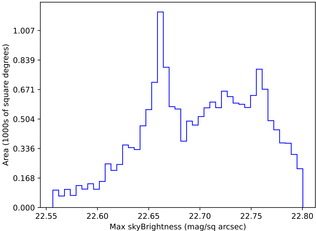
too_ignore_10_4v3.4_10yrs WFD all bands: Max skyBrightness
