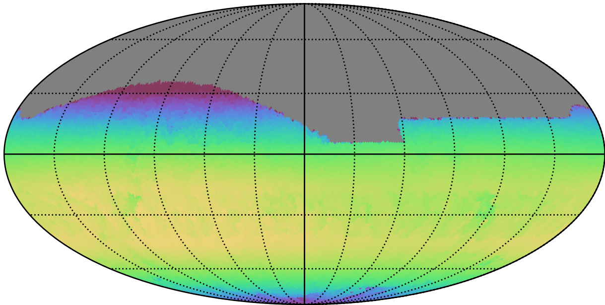
too_ignore_10_4v3.4_10yrs All sky z band: Max skyBrightness
