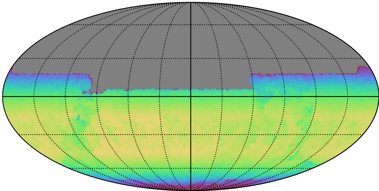
too_ignore_10_4v3.4_10yrs All sky y band: Max skyBrightness
