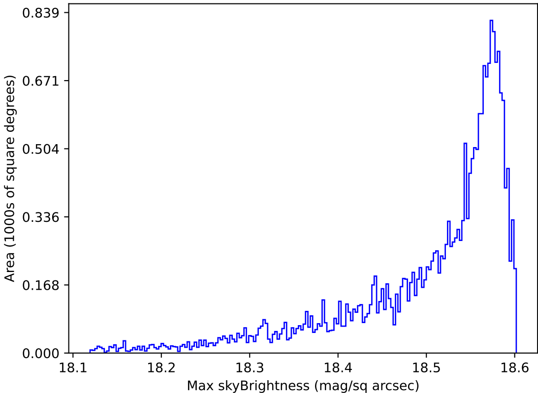
too_ignore_10_4v3.4_10yrs All sky y band: Max skyBrightness
