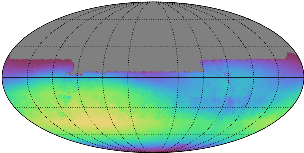
too_ignore_10_4v3.4_10yrs All sky u band: Max skyBrightness
